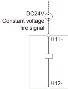
X1-DC24V constant voltage fire module
