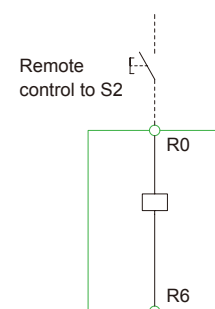
RC2 Remote transfer-to-standby module
