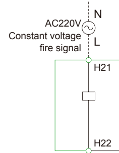
X3-AC220V constant voltage fire module
