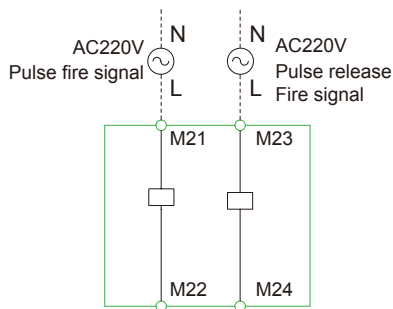
X4-AC220V pulse fire module
