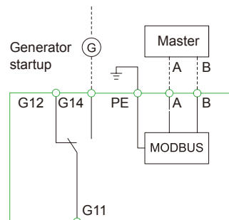
GT Generator starting/cool down + Communication module
