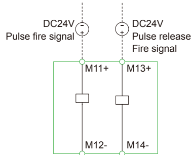
X2-DC24V pulse fire module
